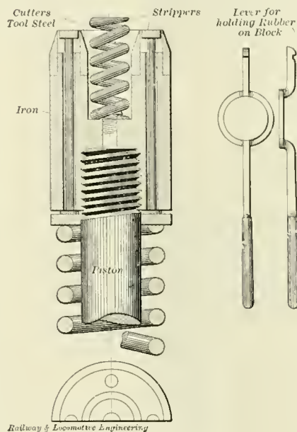
DETAILS OF CUTTER.
